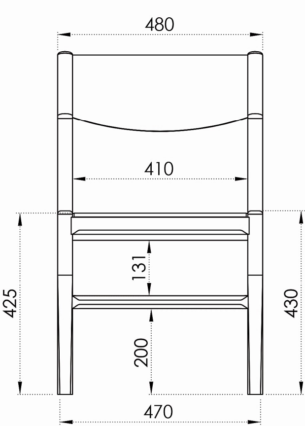
VISTA FRONTAL
