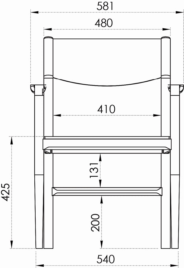
VISTA FRONTAL
